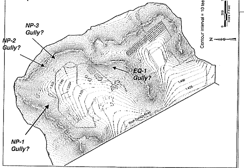
SIBERIA Prediction 10,000 years from now - Gullies are gone and landscape is "rounded"
