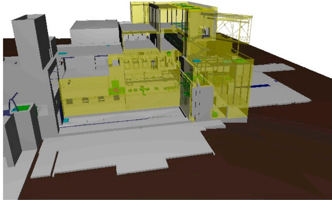
3-D Model of Main Plant Deconstruction (Completed areas in Yellow)
