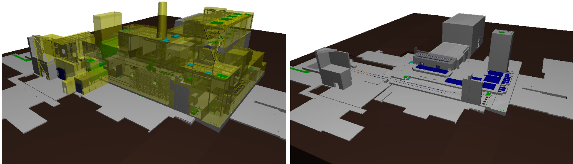
3-D Model of Main Plant Deconstruction (Completed areas in Yellow, Areas remaining in Gray)
