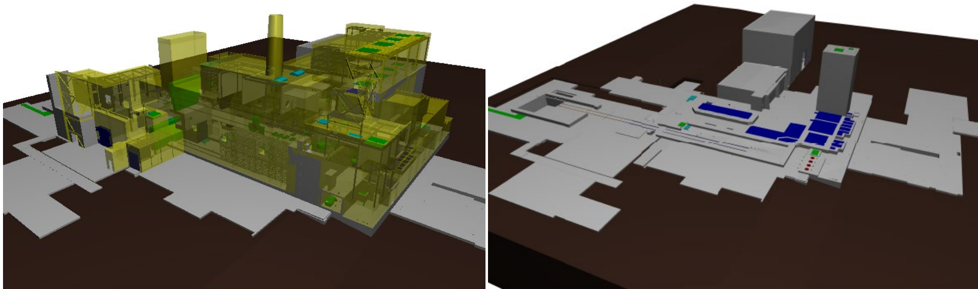
3-D Model of Main Plant Deconstruction (Completed areas in Yellow, Areas remaining in Gray)
