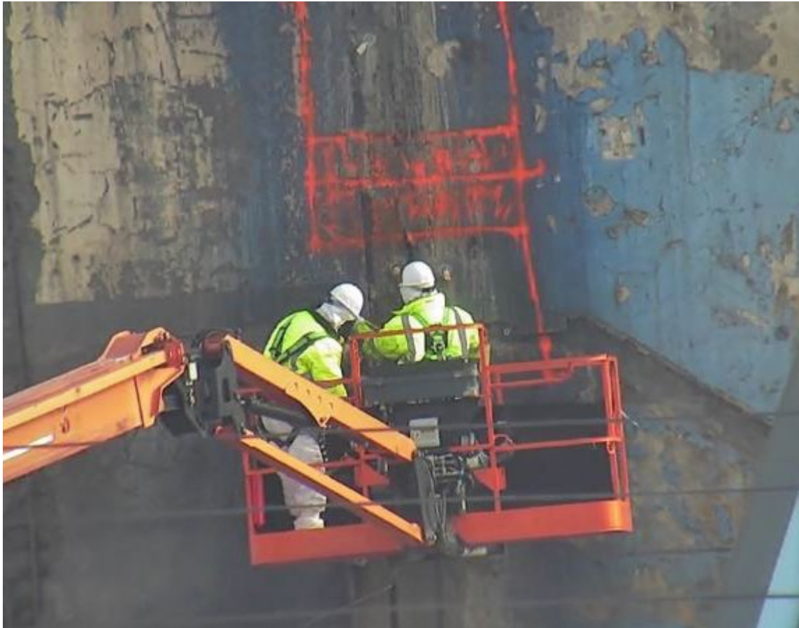
(Left) D&D operators mark demo areas on Off-Gas Cell (Right) Deconstructing OGC with hydraulic hammer
