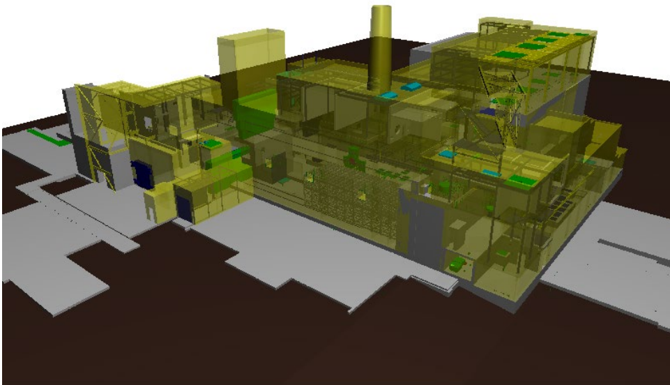
3-D Model of Main Plant Deconstruction (above-grade portion)
