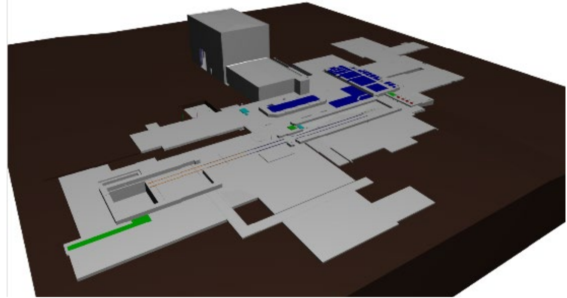
3-D Model of Main Plant Deconstruction (above-grade portion)
